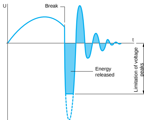
Coil voltage with varistor protection module ( \sim and —)
