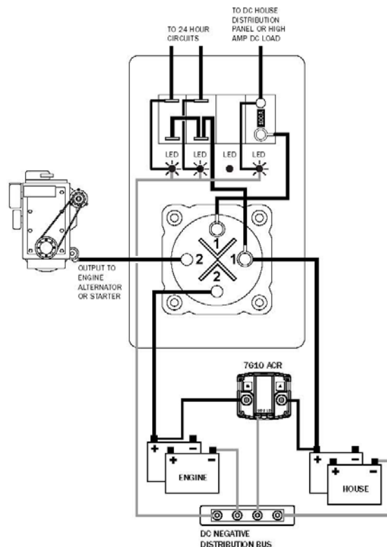
Wiring Diagram Dual Battery Main Distribution Panel PN 8686 Shown
