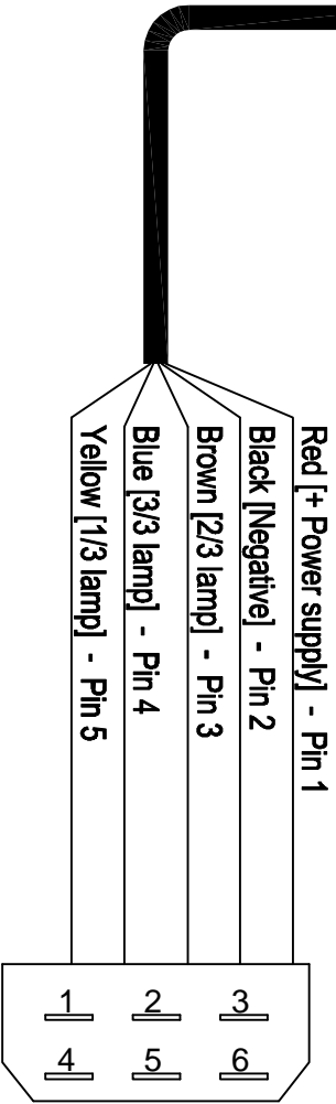
Male contacts side view AMP connector
